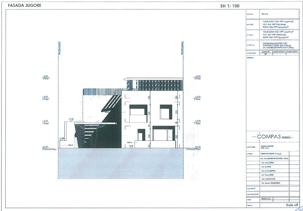
Fig.27 Vila S2/a _ Fasada Jugore
