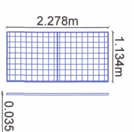
MODULI FOTOVOLTAIK "LR5-72-HBD 550 M 2 SH. 1:50
